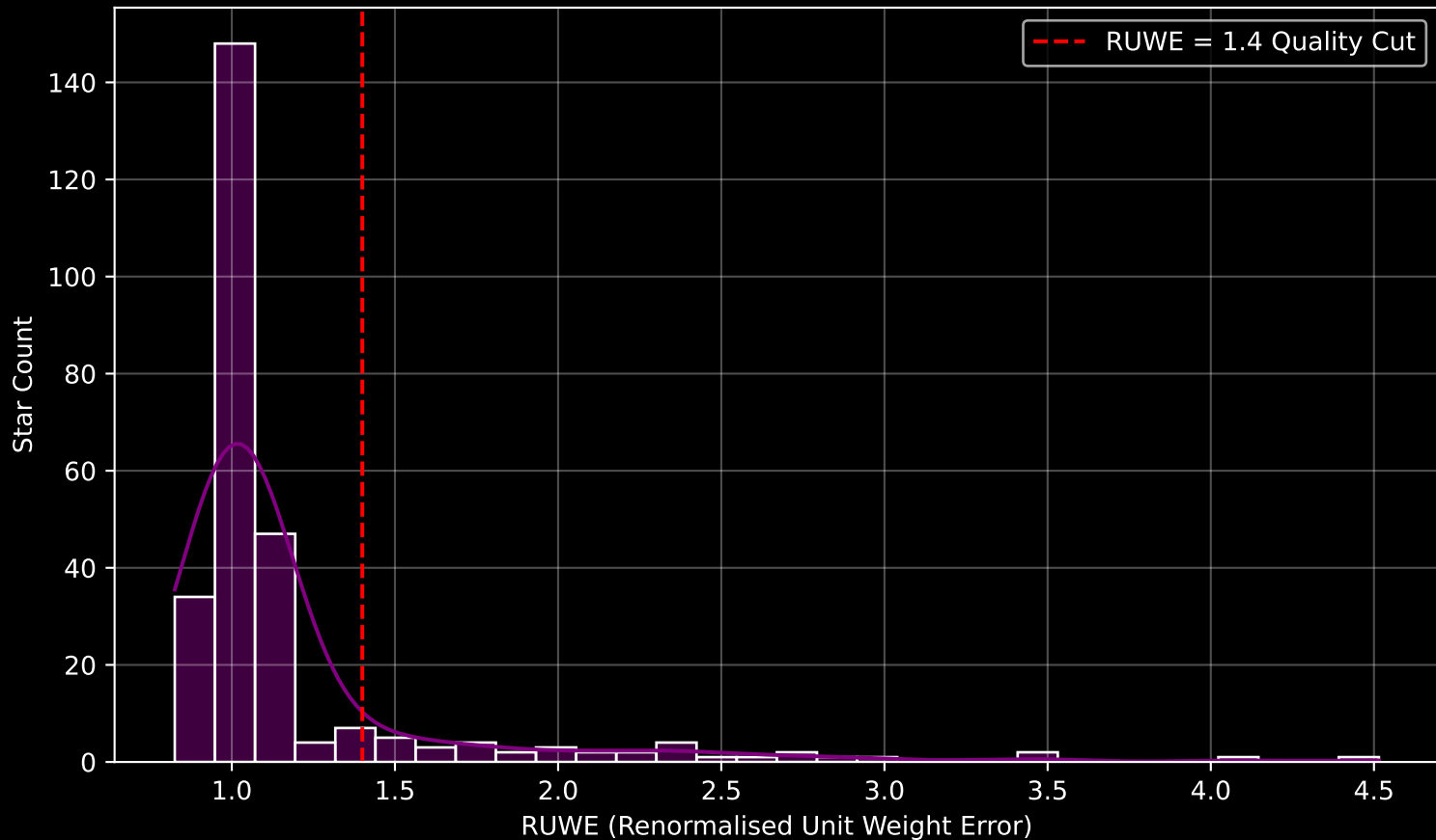
GALAH DR4 Field [1027] RUWE Distribution (n= 275)
