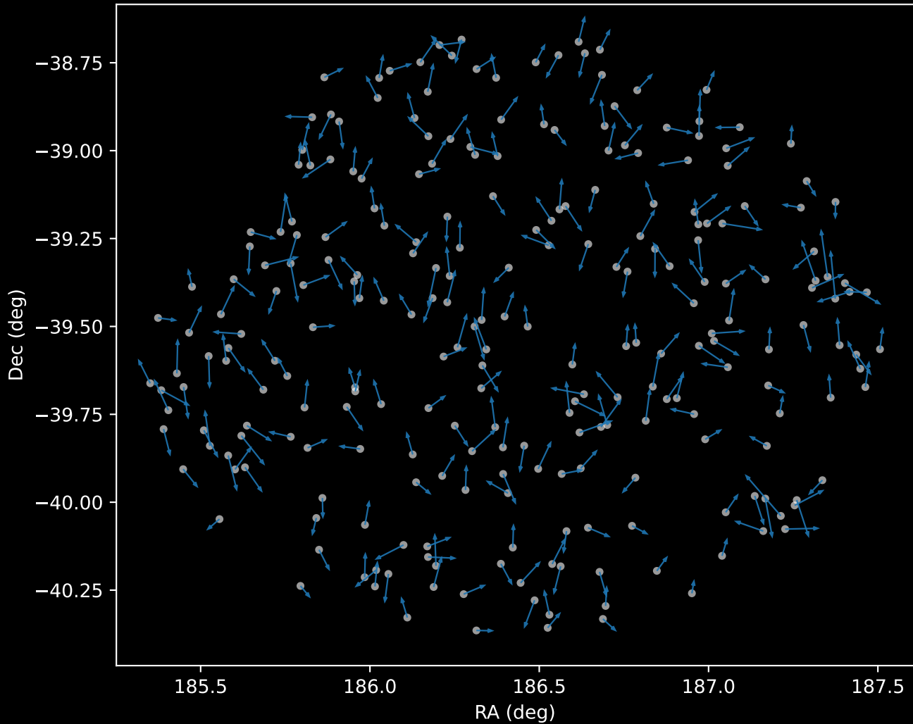
GALAH DR4 Cluster 0 Proper Motion Vectors (n=251)
