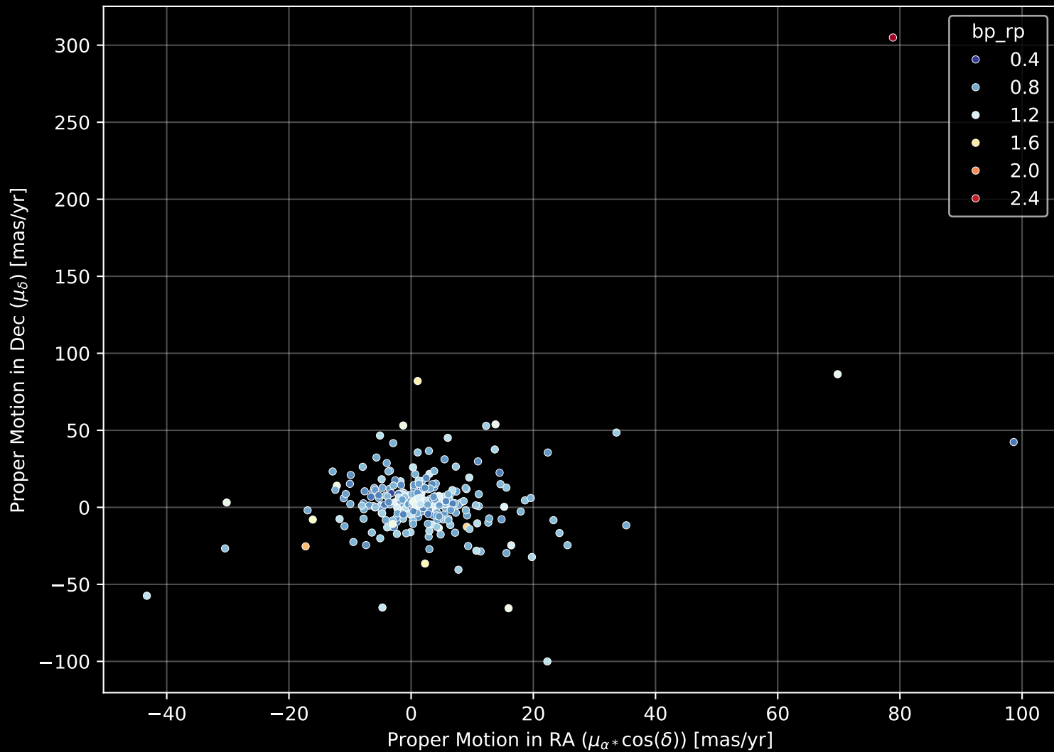
GALAH DR4 Field: [1027] Proper Motion Diagram (n= 287)
