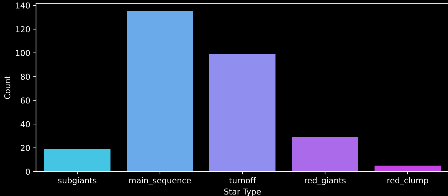
GALAH DR4 Field: [1027] Count plot of Star Type
